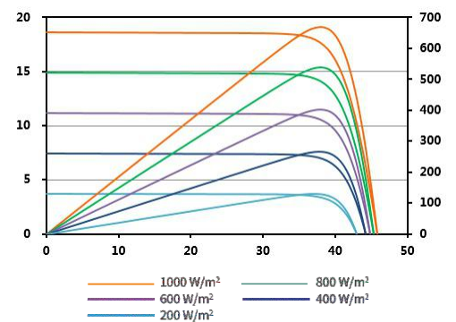
Current (A) Power (W) (A) Power-Voltage&Current-Voltage Curve
