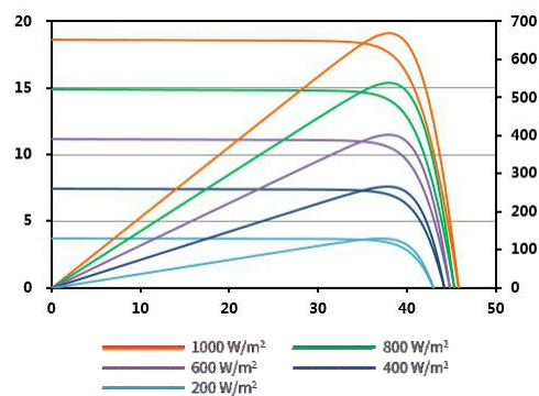
Current (A) Power (W) (A) Power-Voltage&Current-Voltage Curve (W)
