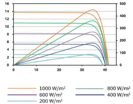
Current (A) Power-Voltage&Current-Voltage Curve Power (W)
