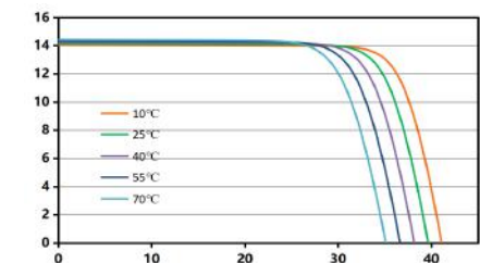
Current (A) Current-Voltage Curve
