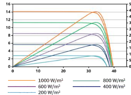
Current (A) Power-Voltage&Current-Voltage Curve Power (W)
