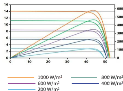
Current (A) Power-Voltage&Current-Voltage Curve (W)
